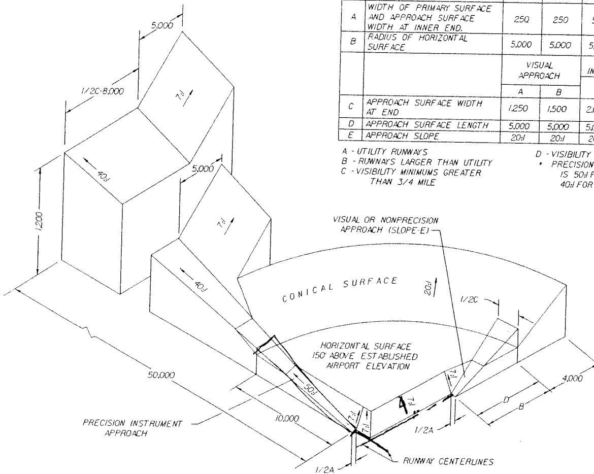
ISOMETRIC VIEW OF AIRPORT IMAGINARY SURFACES
